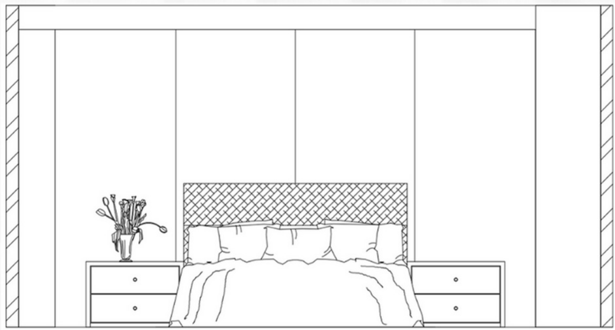
2D ELEVATION DRAFTING
